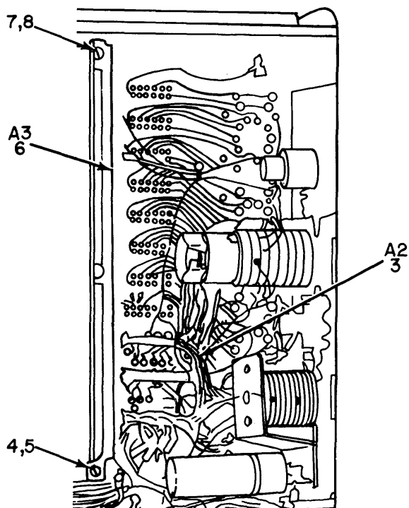
BOTTOM VIEW
