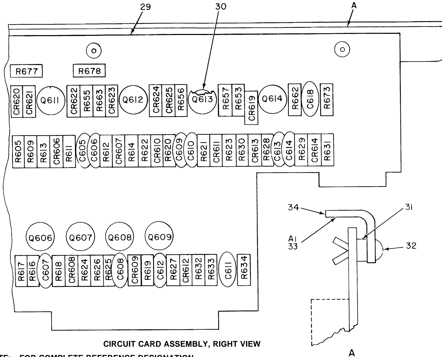
Figure 17. Electronic Digital Readout TD-875A(P)/U 250 KC Decade Board (Sheet 2 of 3).
