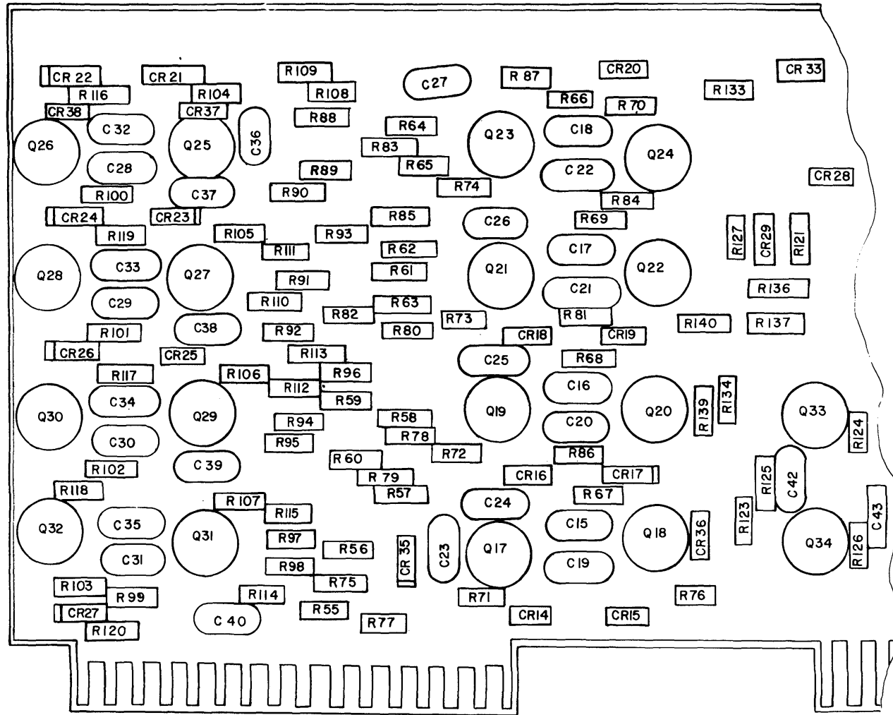
COMPONENT BOARD LEFT VIEW
