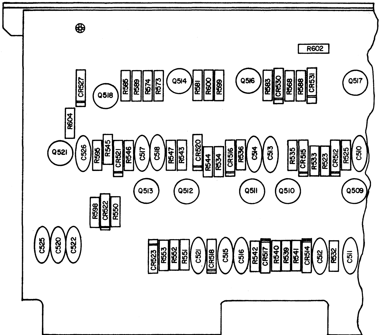
CIRCUIT CARD ASSEMBLY, LEFT VIEW
