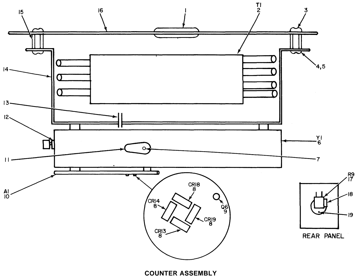
Figure 31. Electronic Digital Readout TD-875A(P)/U Electronic Components (Sheet 1 of 2).
