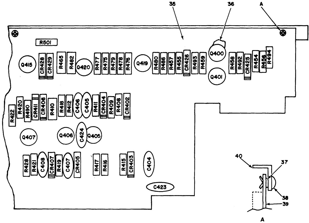
CIRCUIT CARD ASSY, RIGHT VIEW
