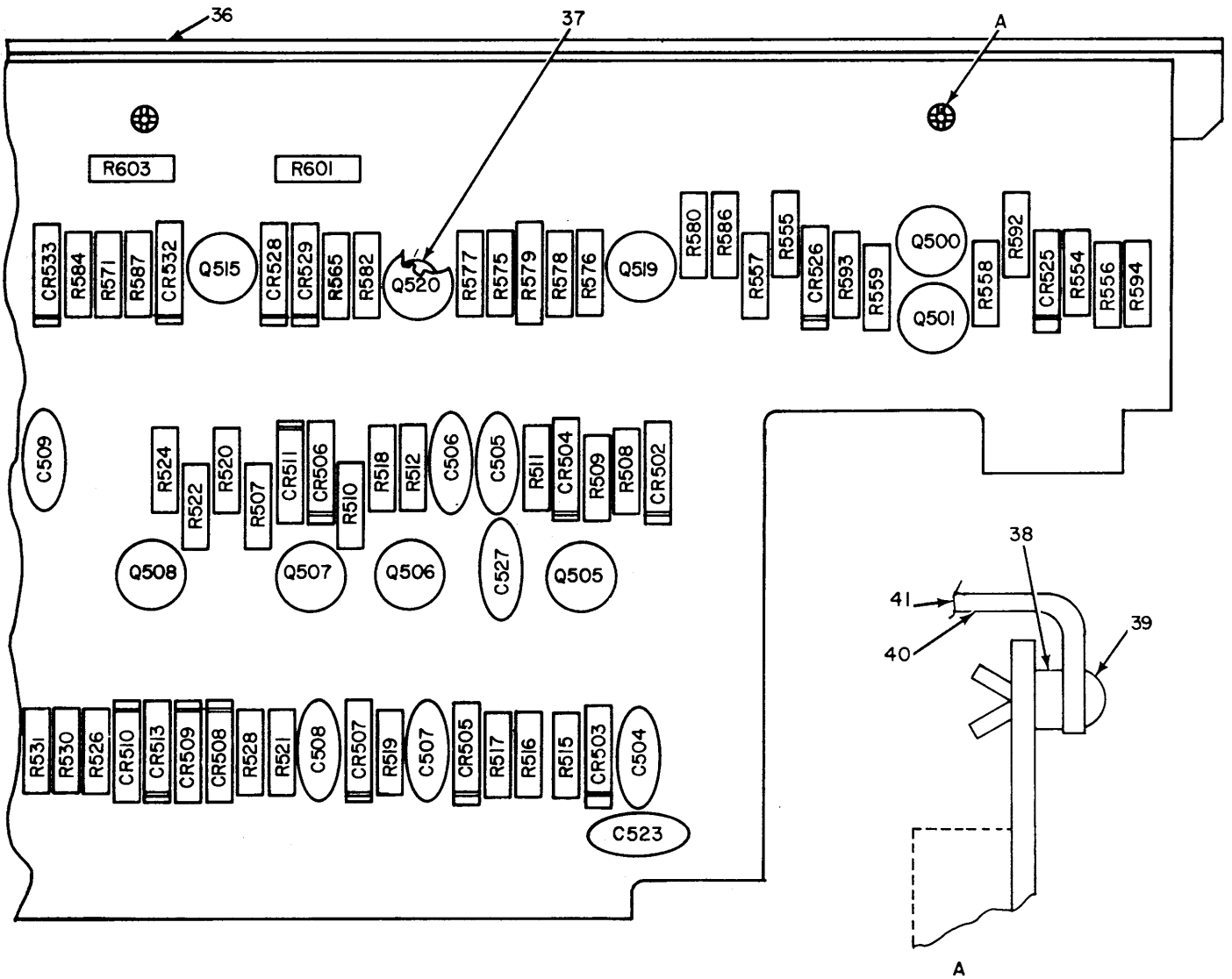
CIRCUIT CARD ASSEMBLY, RIGHT VIEW
