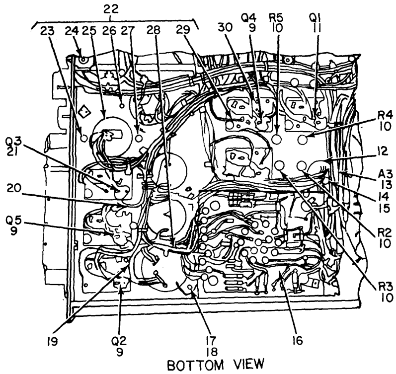
Figure 11. Electronic Digital Readout TD-875A(P)/U Power Supply Chassis.
