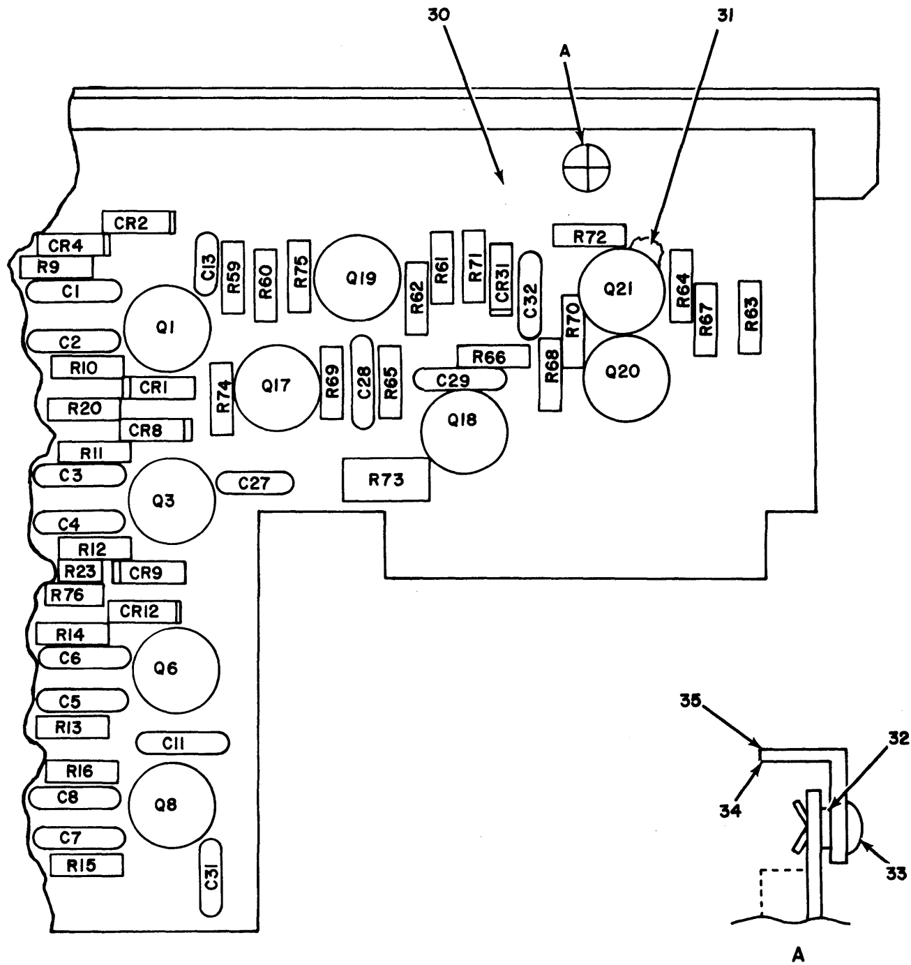
RIGHT PARTIAL VIEW
