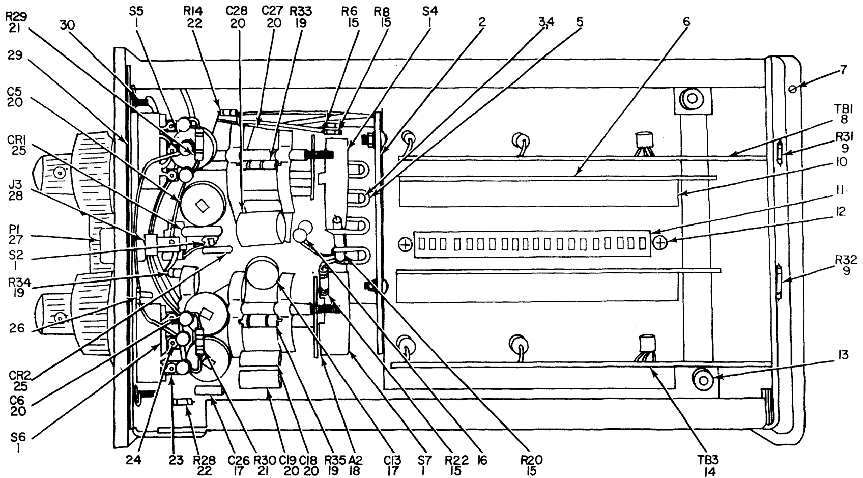
Figure 37. Converter Frequency Elec. Counter CV-2349/U Electronic Chassis Assy.
