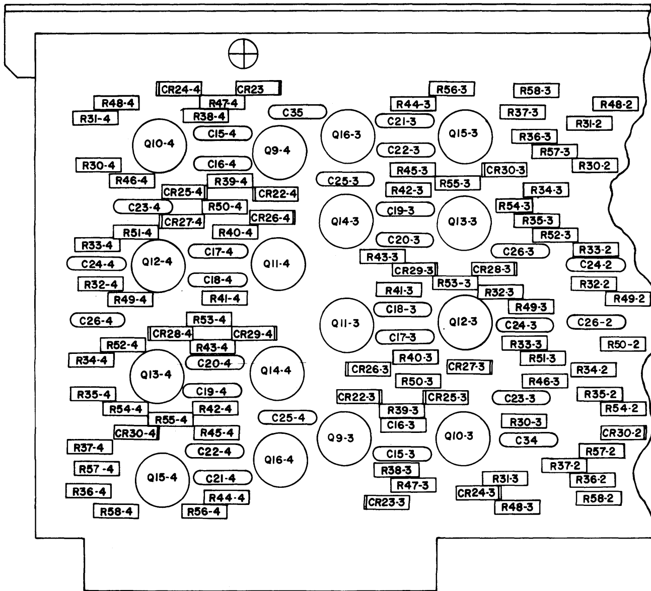
LEFT PARTIAL VIEW
