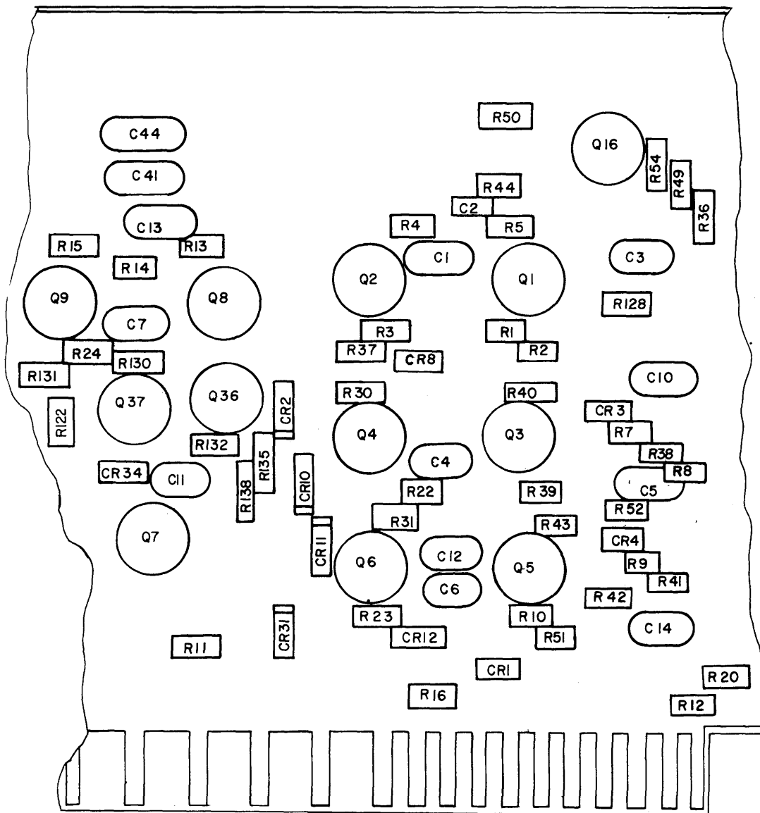
COMPONENT BOARD CENTER VIEW
