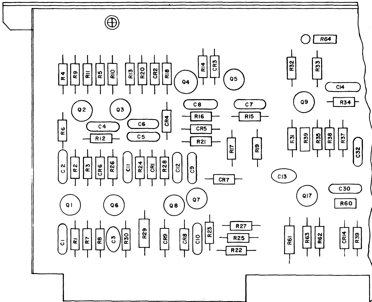
LEFT PARTIAL VIEW
