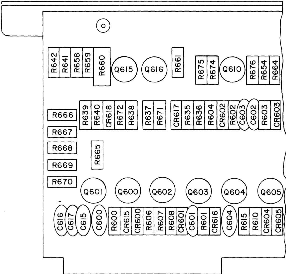
CIRCUIT CARD ASSEMBLY, LEFT VIEW
