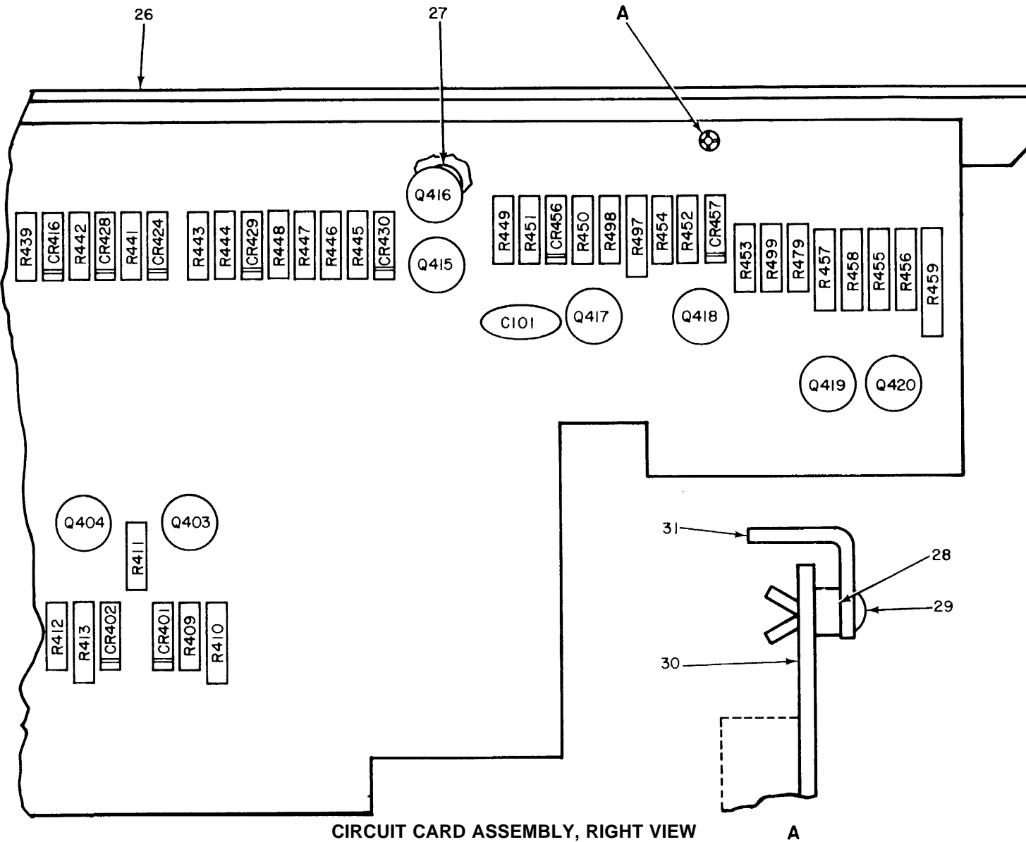
Figure 19. Electronic Digital Readout TD-875A(P)/U 50 Megahertz Readout Assembly (Partial View) (Sheet 2 of 3).
