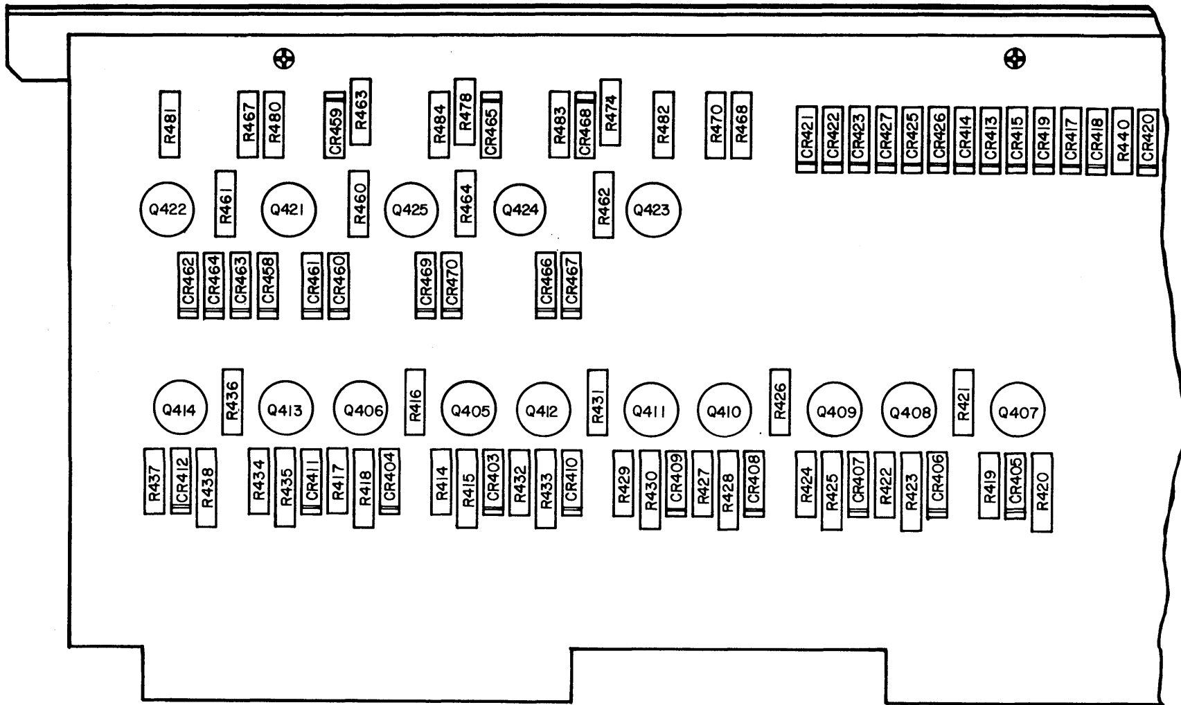
CIRCUIT CARD ASSEMBLY, LEFT VIEW
