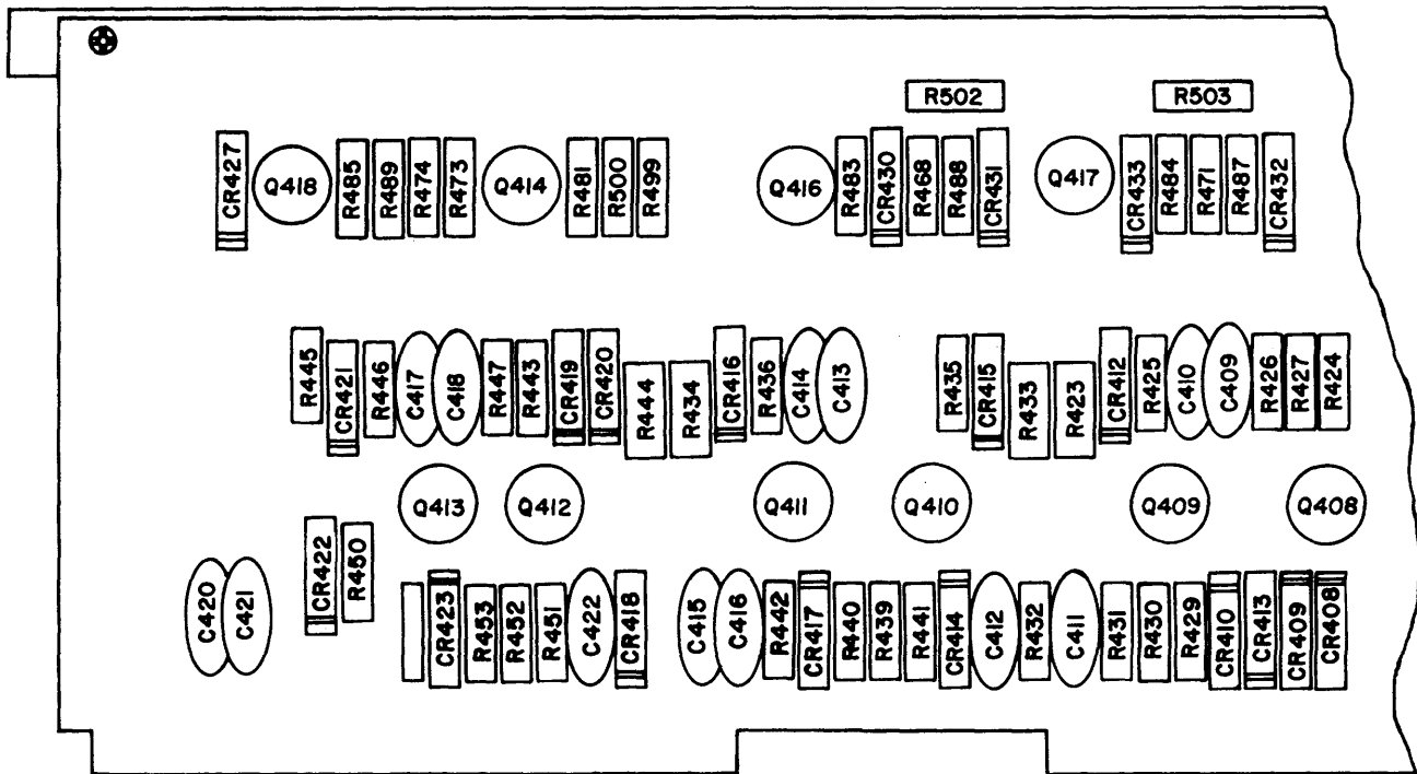
CIRCUIT CARD ASSY, LEFT VIEW
